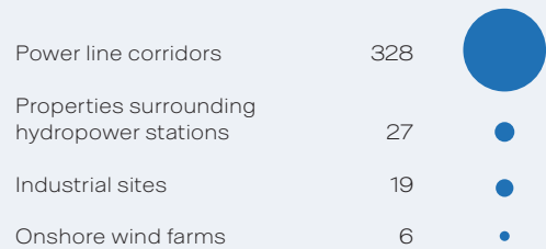
Figure 1. Vattenfall's terrestrial static biodiversity footprint, in MSA.km 2
